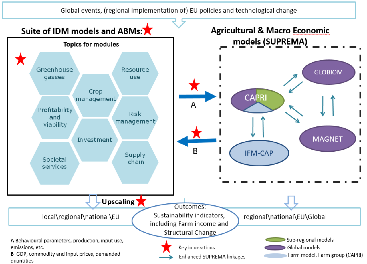
Figure 5 MIND STEP model toolbox: Integration of Individual Decision Making (IDM) models and current models.
