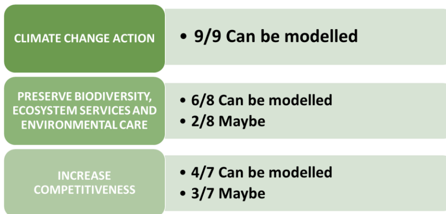
Figure 4 Group of scenarios that can be modelled.
