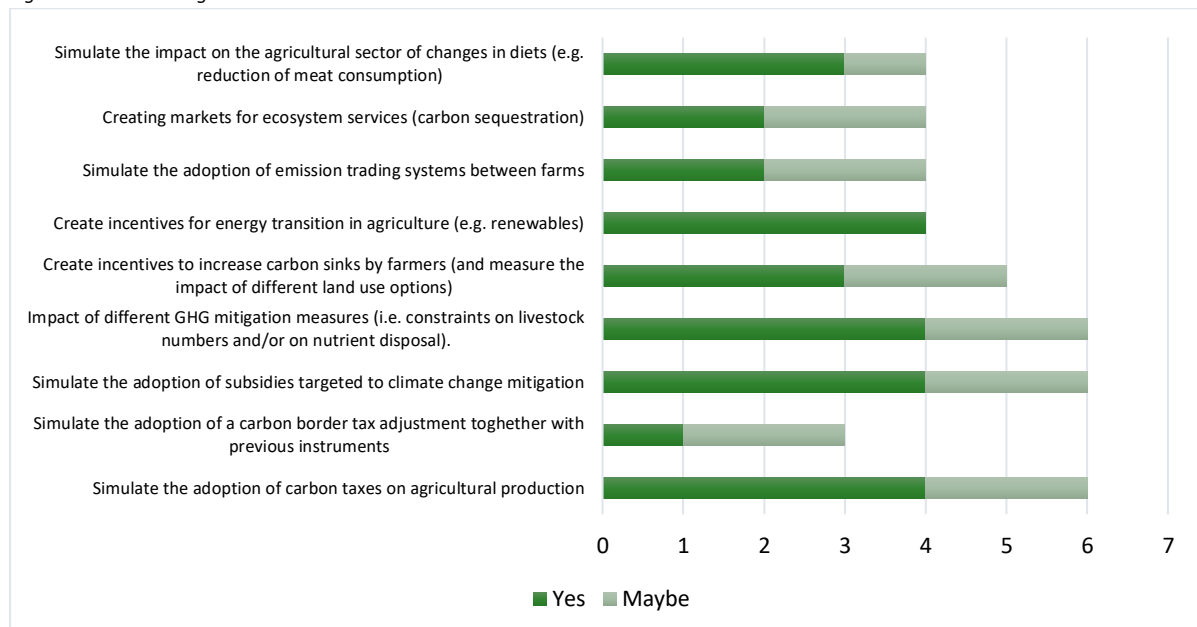
Figure 1 Climate change scenarios that can be modelled.
