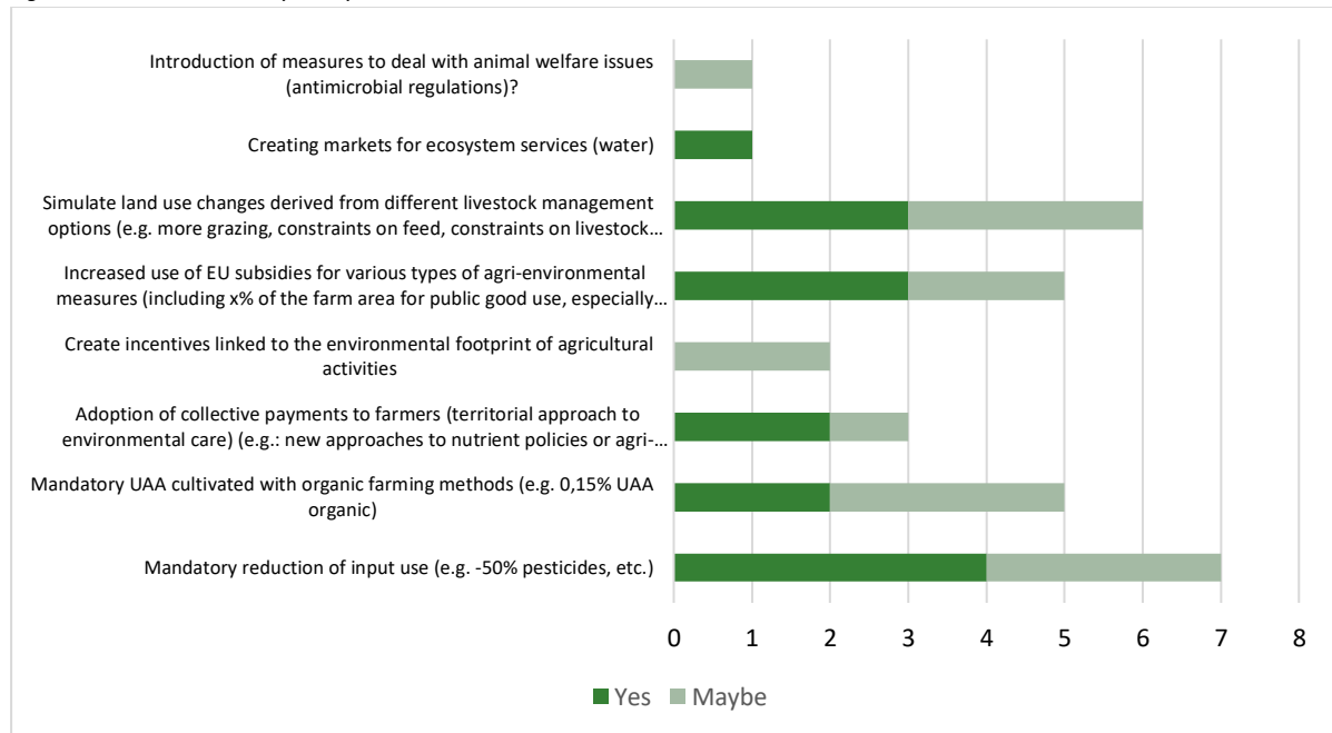
Figure 2 Preserve Biodiversity, Ecosystem Services and Environmental Care scenarios that can be modelled.
