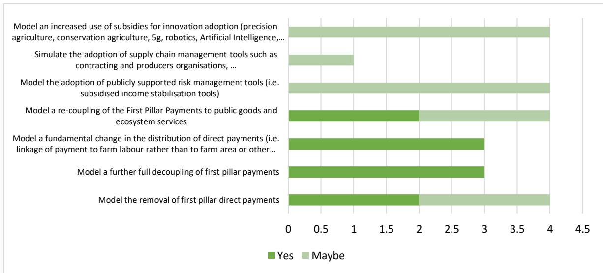
Figure 4 summarizes the number of scenarios that can be modelled according to each group.
